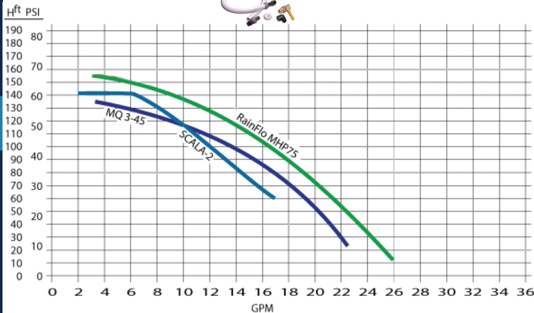
RainFlo MHP75 Performance Chart
