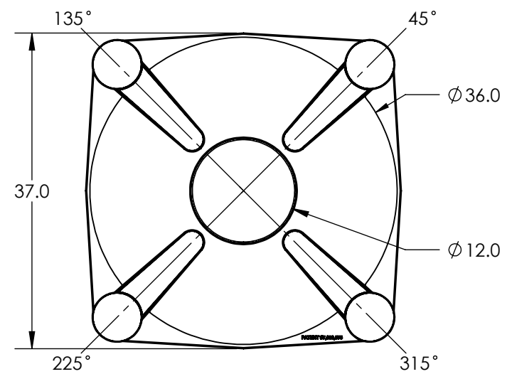
18" LEG VERSION P/N: 1730001N
