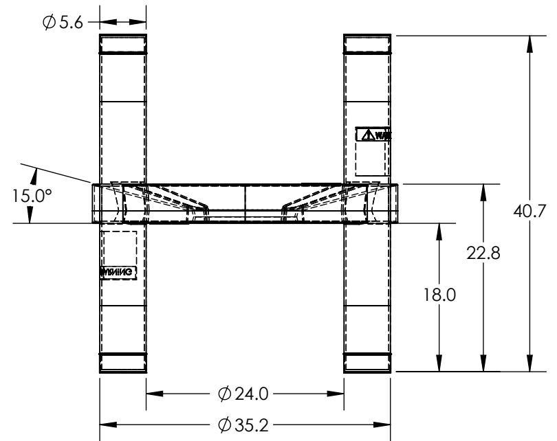
18" LEG VERSION P/N: 1730001N
