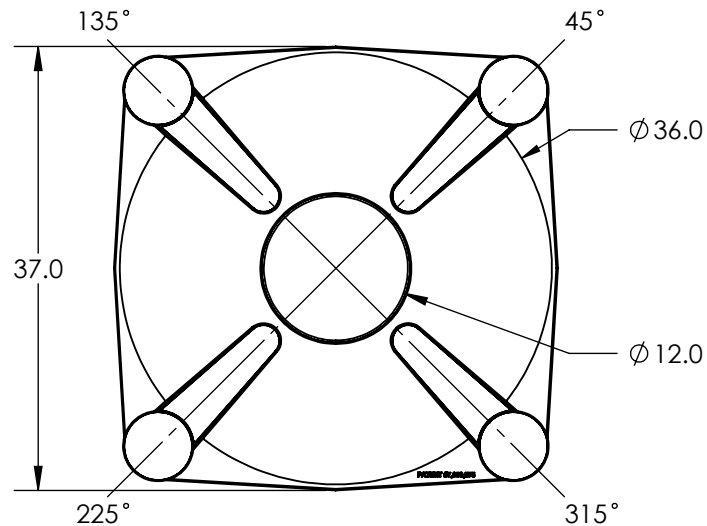
12" LEG VERSION P/N: 1730000N
