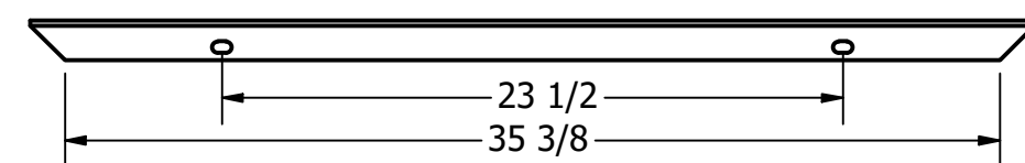
ANGLE FOR 3135 TANK SCALE 1:8
