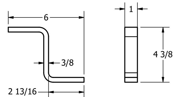
LADDER BRACKET SCALE 1:4
