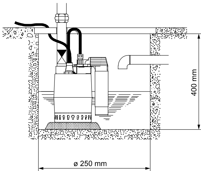
Minimum well dimensions, UNILIFT KP-AV
