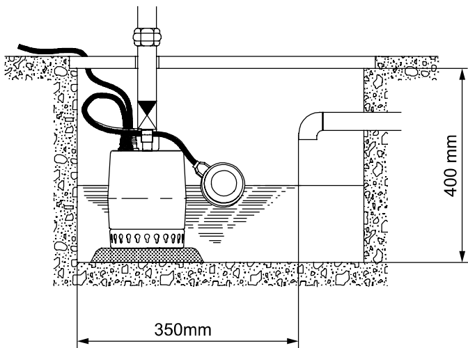
Minimum well dimensions, UNILIFT KP-A
