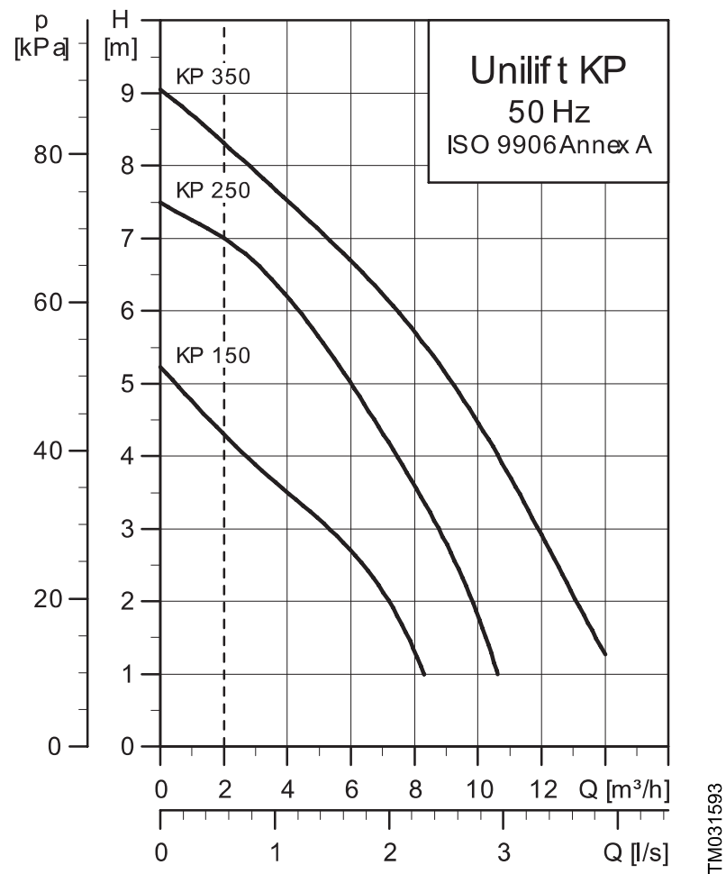
Performance curves UNILIFT KP 50 Hz
