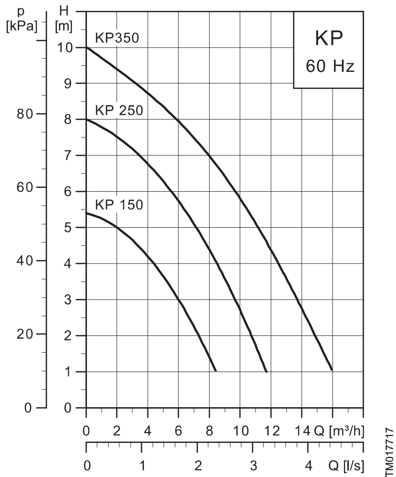
Performance curves UNILIFT KP 60 Hz
