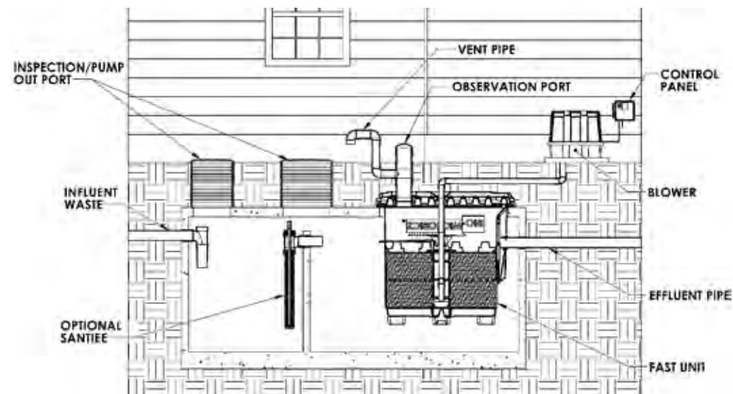
LID INSTALLATION OPTION*
