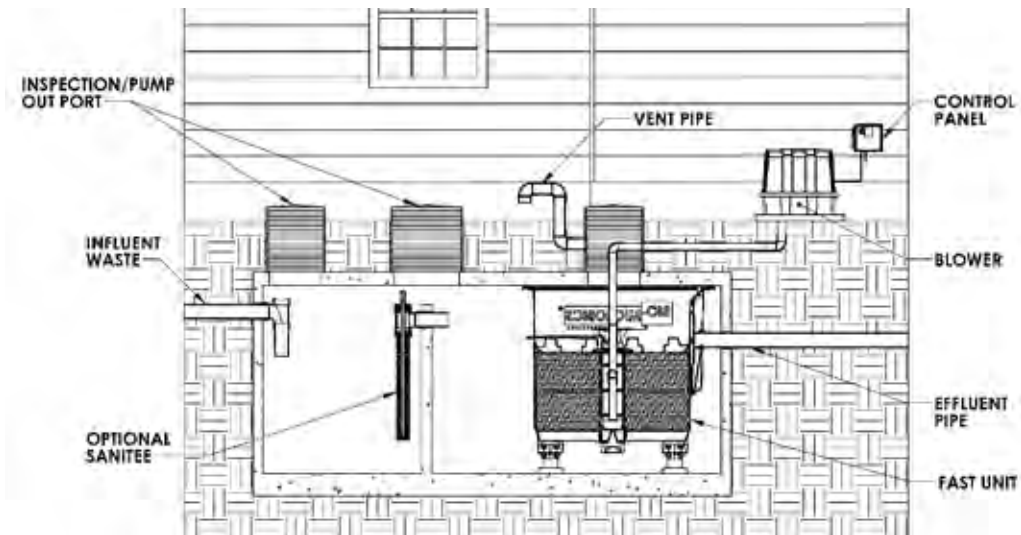
FOOT INSTALLATION OPTION
